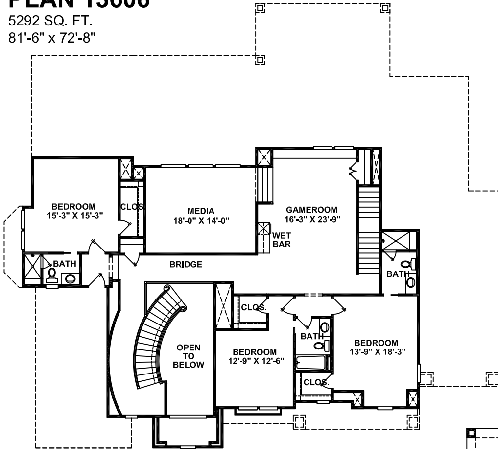
SECOND FLOOR
