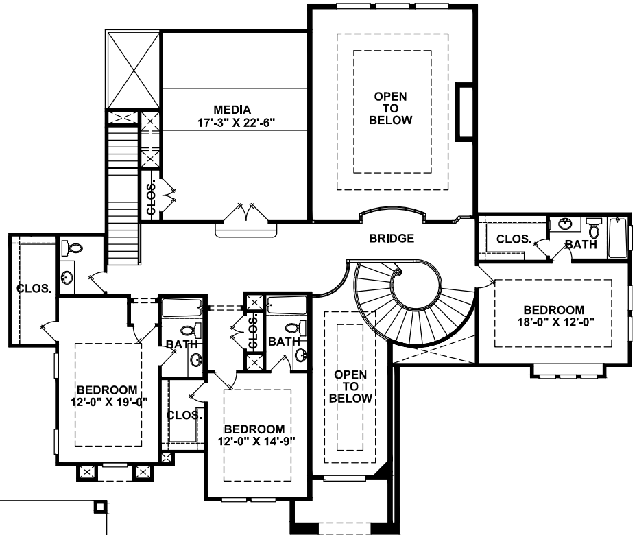
SECOND FLOOR
