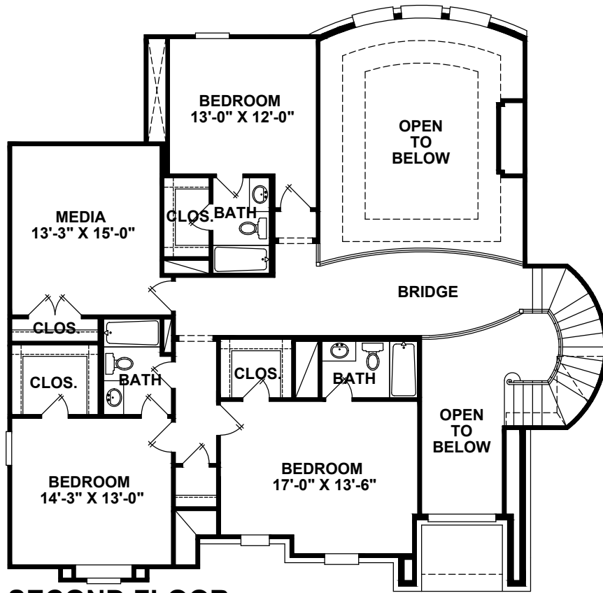
SECOND FLOOR
