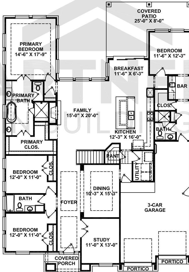
FIRST FLOOR
