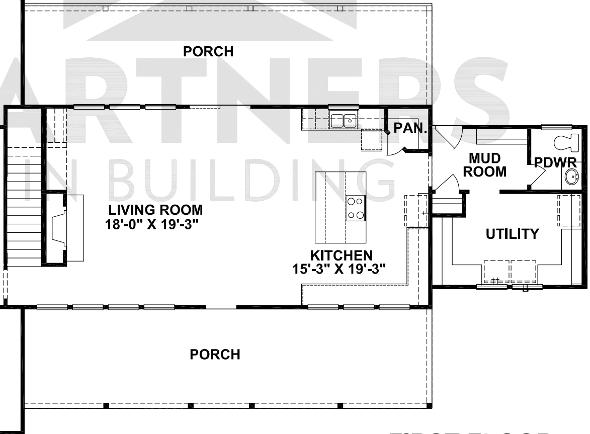
FIRST FLOOR
