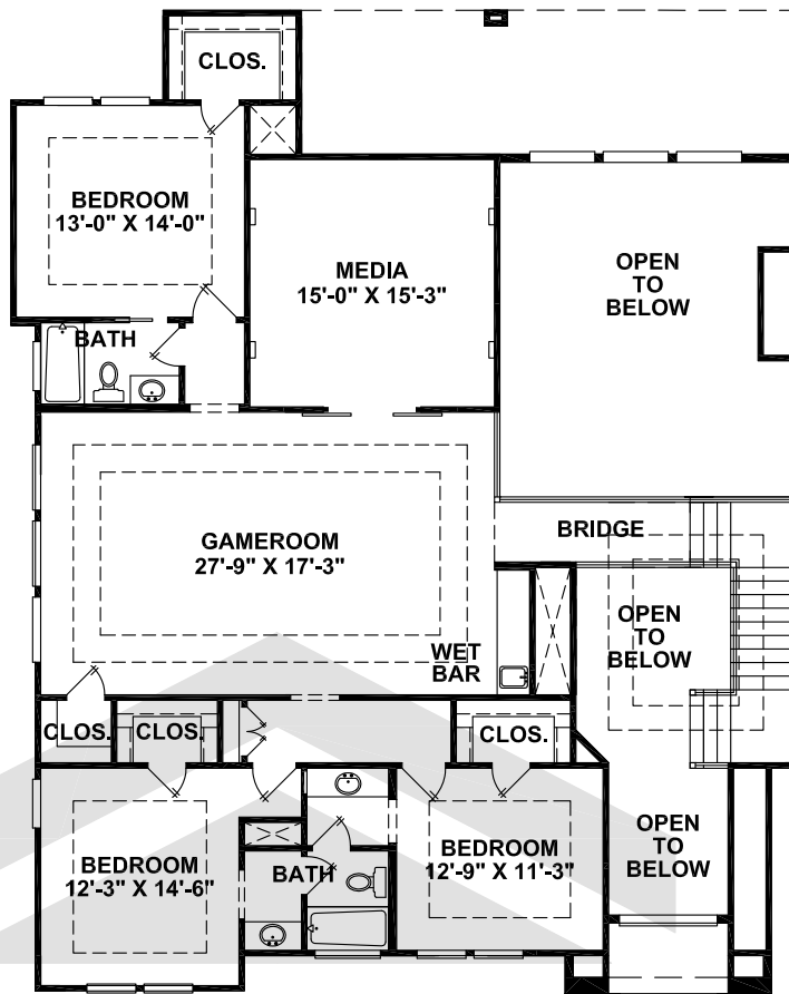
SECOND FLOOR
