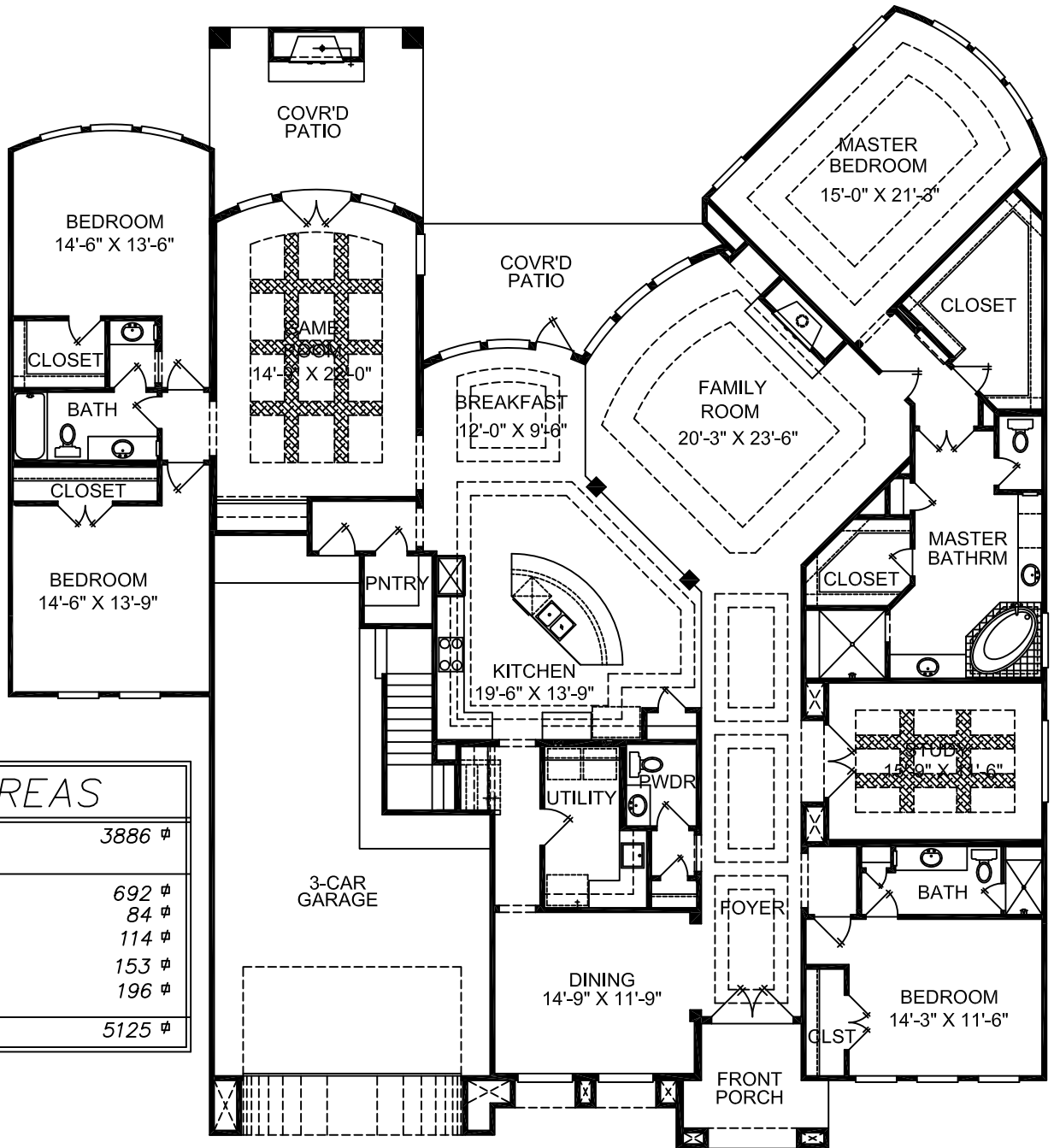
FIRST FLOOR
